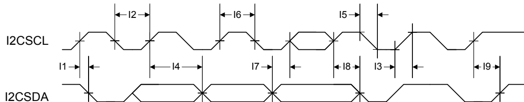
Figure 26-16. I 2 C Timing
