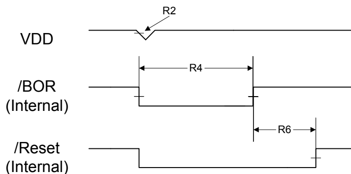
Figure 26-7. Software Reset Timing
